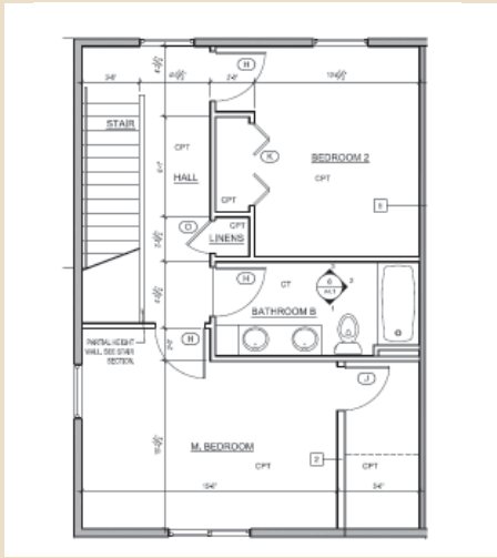
Jackson Model - Second Floor
