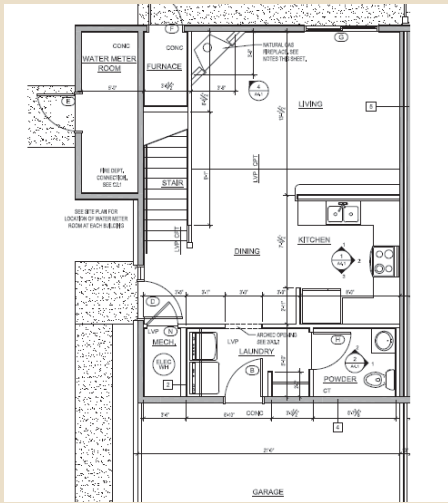
Jackson Model - First Floor
