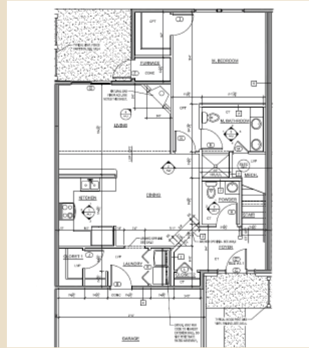
Logan Model - First Floor
