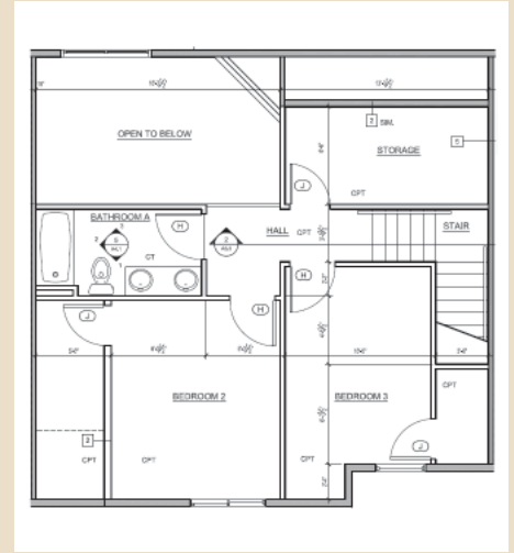
Logan Model - Second Floor
